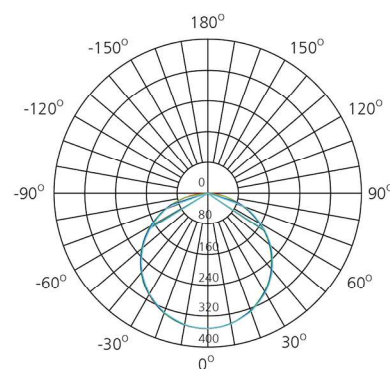
AVERAGE BEAM ANGLE (50%): 115.5 DEG
