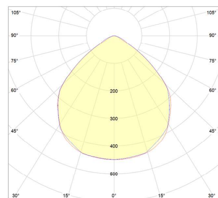
cd/klm: c0-180 c90-270
