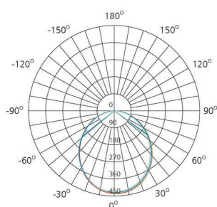
cd/klm: c0-180 c90-270
